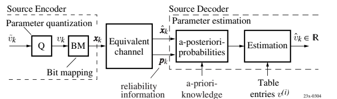
Figure 5: Error concealment by soft decision source decoding.
