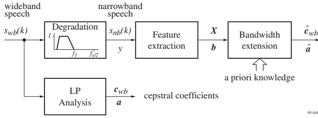
Figure 9: Model of bandwidth extension by conditional estimation. Correspondence with respect to Fig. 2a: \mathbf{c}_{wb} = \mathbf{a} , \mathbf{X} = \mathbf{b} , \hat{\mathbf{c}}_{wb} = \hat{\mathbf{a}} (vectors); wb=wideband; nb=narrowband
