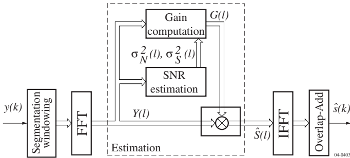
Figure 3: Single microphone noise reduction system.
