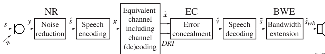
Figure 1: Speech communication system.
