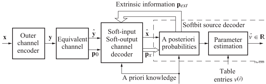
Figure 7: The concept of iterative source–channel decoding (“Turbo error-concealment” [18]).
