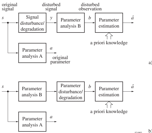
Figure 2: Conditional estimation in a parameter domain using a priori knowledge
