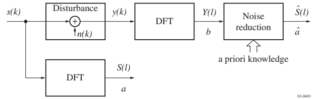
Figure 4: Model of noise suppression by conditional estimation. Correspondence with respect to Fig. 2a:
