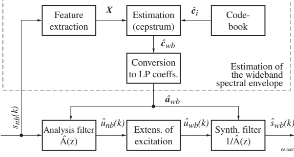
Figure 8: Block diagram of the BWE algorithm
