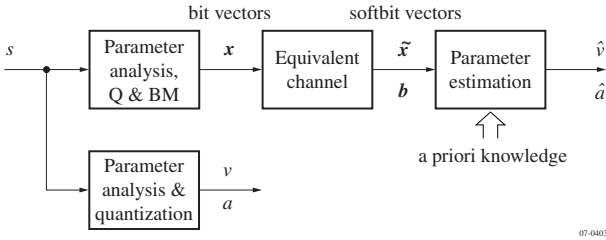
Figure 6: Model of soft decision error concealment by conditional estimation. Correspondence with respect to Fig. 2b: v = a (quantized parameter), \tilde{\mathbf{x}} = \mathbf{b} (softbit vector), \hat{v} = \hat{a} .
