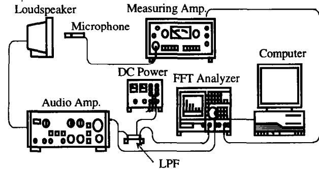
Fig. 3 Automatic measuring system of second-order VFR.
