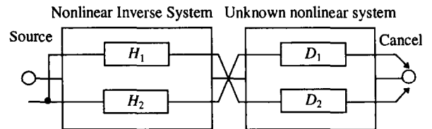
Fig. 5 The block diagram of tandem connection of the nonlinear inverse system and the unknown nonlinear system.
