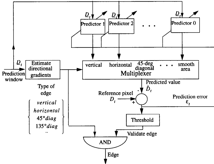
Figure 1: Edge detection based on adaptive context prediction residuals
