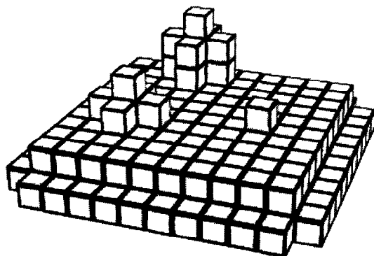
Figure 6. The result of performing a dilation of the image umbra in Figure 4 with the structuring element in Figure 5 presented as an Umbra. Observe the bevelling around the edge of the image.
