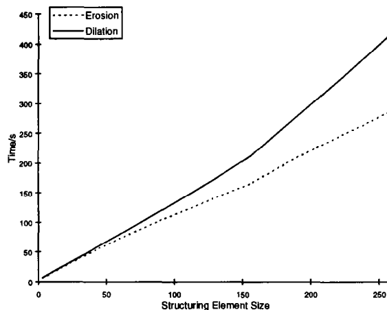
Figure 1. Graph of Time to dilate and erode an 864 black square image, using the Brute Force Morphology method with various sizes of 1D structuring element.
