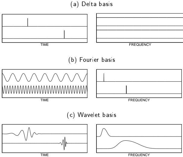
Figure 2: Comparison of different bases \{\mathbf{b}_j\} for nonlinear signal processing. The choice of basis employed in the linear front end of the NST of Figure 1 determines in which domain we represent signal interactions. Consider a second-order NST, which generates squares \beta_j^2 and cross-products \beta_i\beta_j of the signal coefficients. We illustrate two basis elements \mathbf{b}_i and \mathbf{b}_j from three different bases, in both the time domain and the frequency (squared magnitude) domain. In the delta basis, each \mathbf{b}_j is a unit pulse, so \beta_j is simply a sample of the signal. The corresponding NST represents coupling between different time lags of the signal. In the Fourier basis, each \mathbf{b}_j is a sinusoid, so \beta_j is a Fourier coefficient of the signal. The corresponding NST represents intermodulations between different frequencies. In the wavelet basis, each \mathbf{b}_j is localized in both time and frequency simultaneously, so \beta_j measures the time-frequency content of the signal. The corresponding NST represents coupling between different localized wavelet atoms.
