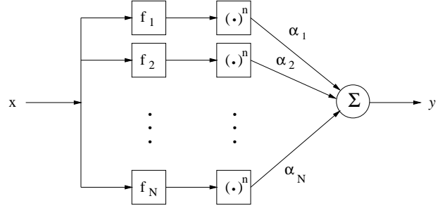
Figure 3: Volterra filter realization using a summing node NST.
