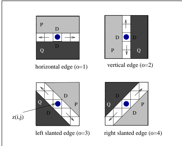
Figure 1: MSP-RoA scheme
